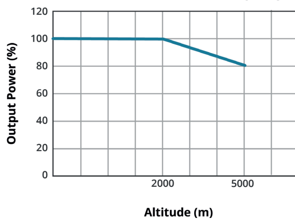
ALTITUDE DERATING CURVE (25°C)
