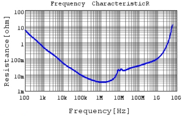
GRM21BR61A225KA01 R DCOV, 25degC
