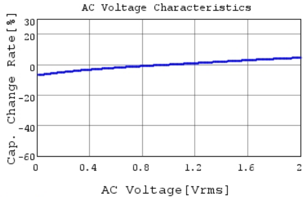
GRM21BR61A225KA01 C-AC Voltage capchange, DC
