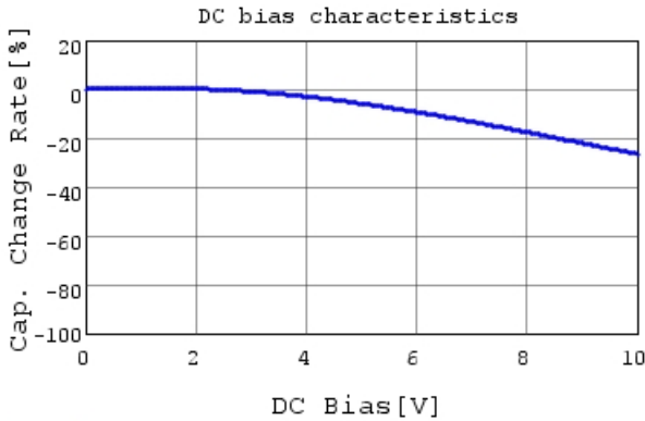
GRM21BR61A225KA01 C-DC bias capchange, 25.0c
