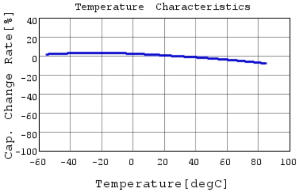
GRM21BR61A225KA01 C-Temp. capchange, DC0.0V,
