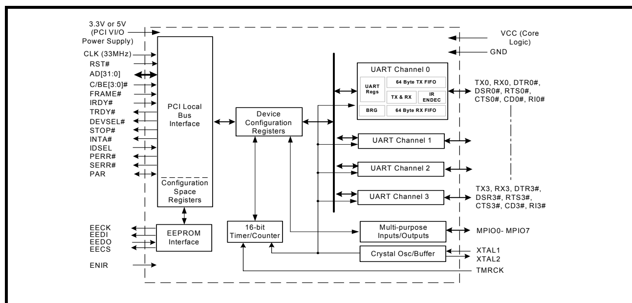
FIGURE 1. BLOCK DIAGRAM
