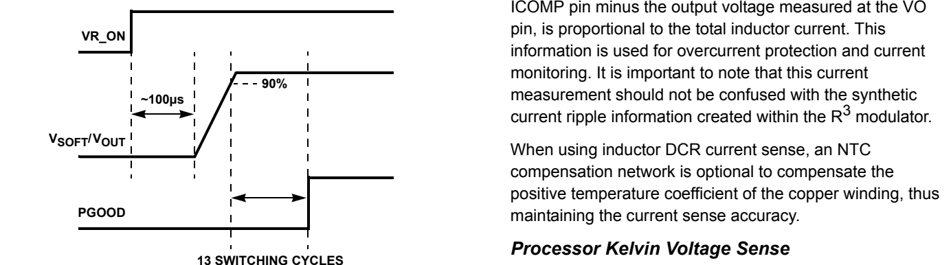
FIGURE 4. ISL6263C START-UP TIMING
