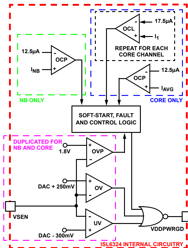
FIGURE 13. POWER-GOOD AND PROTECTION CIRCUITRY
