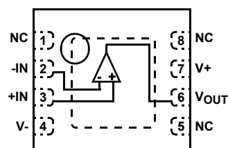
ISL28117 (8 LD TDFN) TOP VIEW
