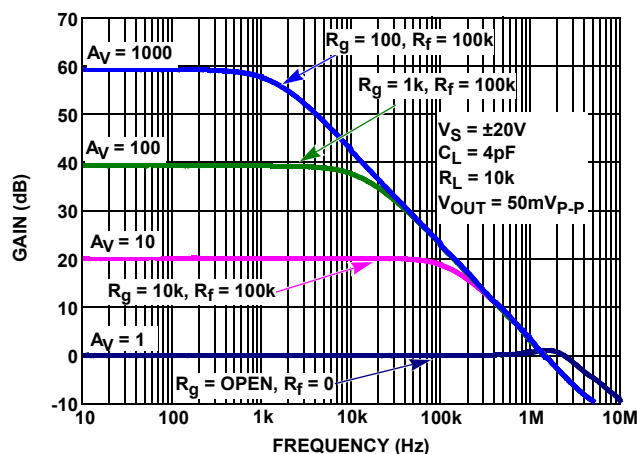
FIGURE 42. FREQUENCY RESPONSE vs CLOSED LOOP GAIN
