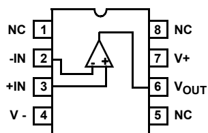
ISL28117 (8 LD SOIC, MSOP) TOP VIEW
