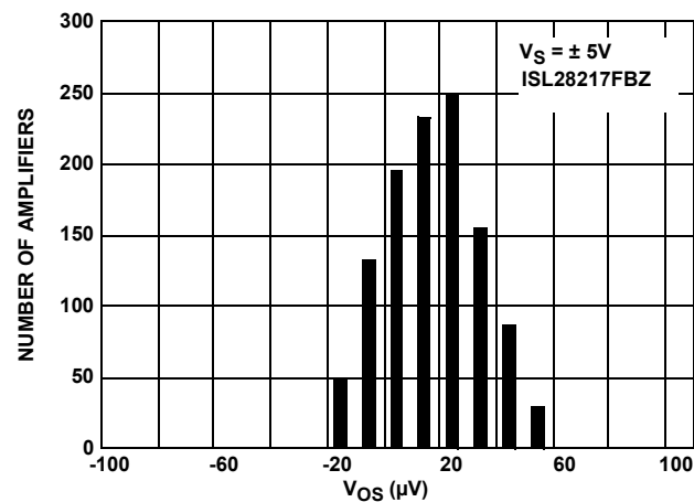
FIGURE 6. V_{OS} DISTRIBUTION FOR GRADE C
