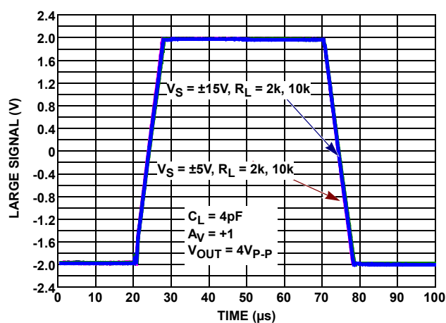
FIGURE 48. LARGE SIGNAL TRANSIENT RESPONSE vs R_L V_S = \pm 5V , \pm 15V
