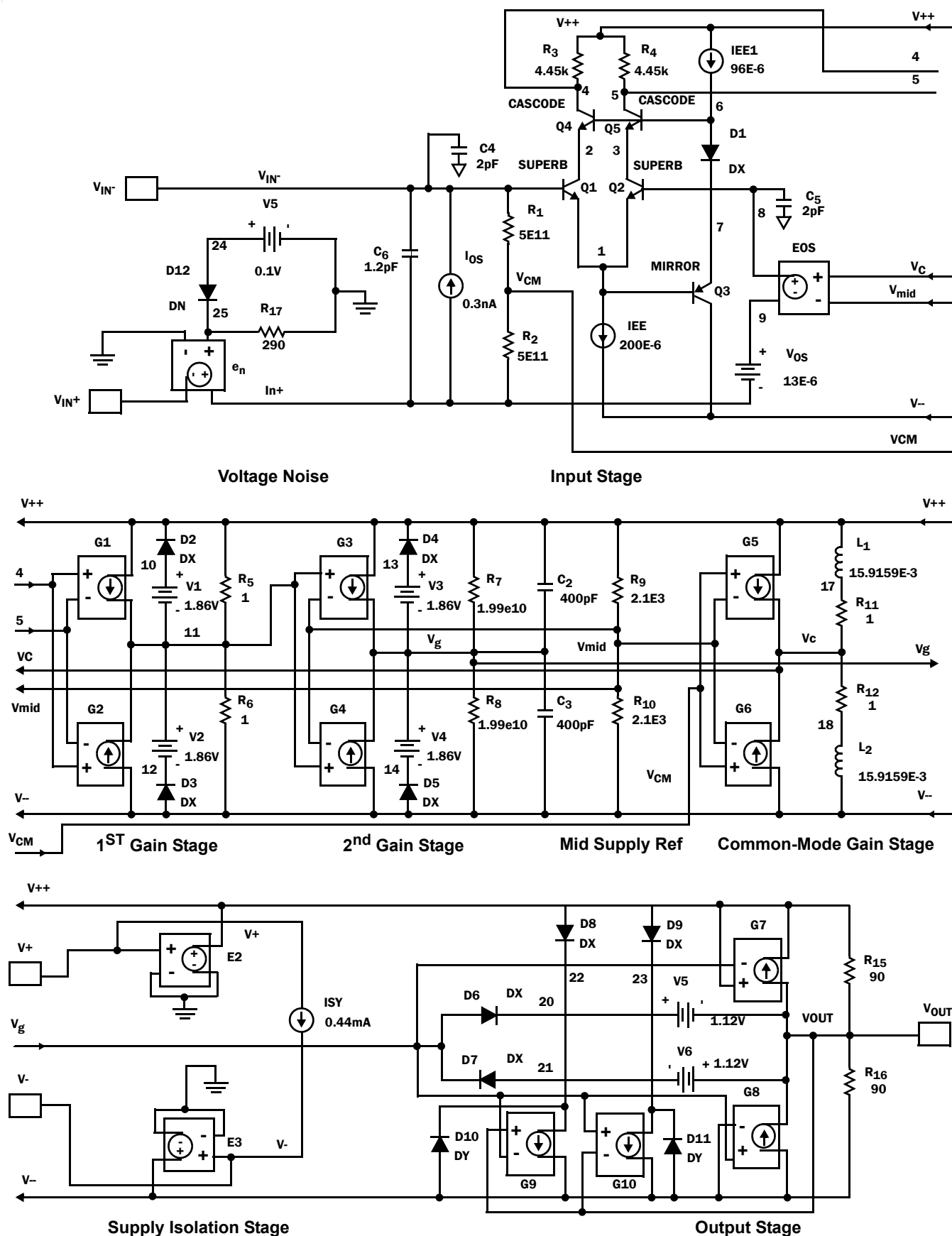
FIGURE 56. SPICE SCHEMATIC
