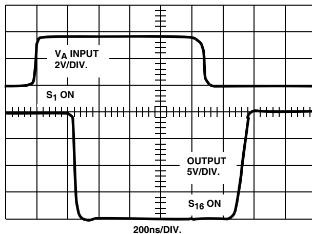
FIGURE 5D. WAVEFORMS
