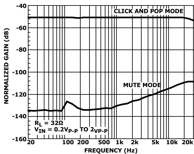
FIGURE 14. OFF-ISOLATION
