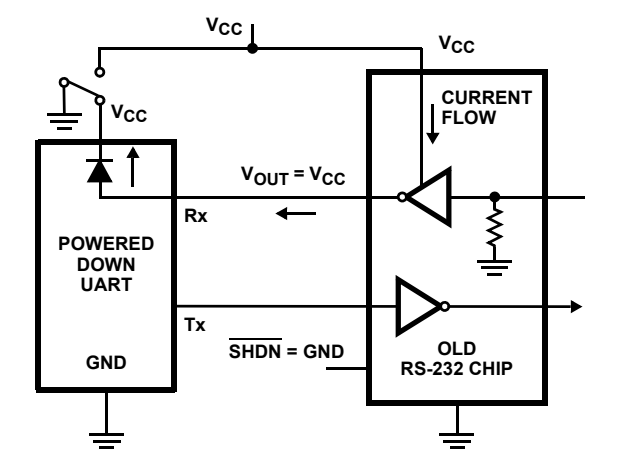
FIGURE 3. POWER DRAIN THROUGH POWERED DOWN PERIPHERAL
