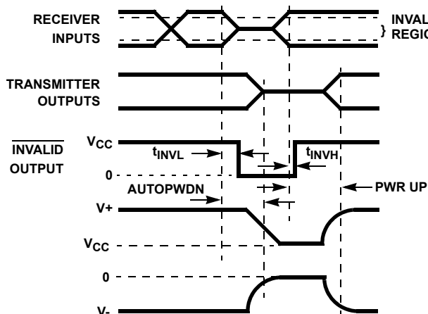
FIGURE 8. AUTOMATIC POWER-DOWN AND \overline{\text{INVALID}} TIMING DIAGRAMS
