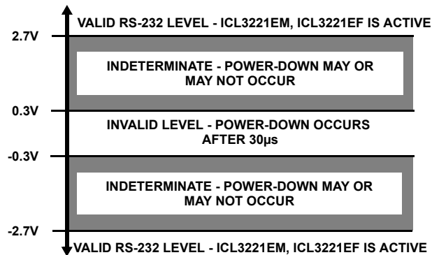
FIGURE 7. DEFINITION OF VALID RS-232 RECEIVER LEVELS
