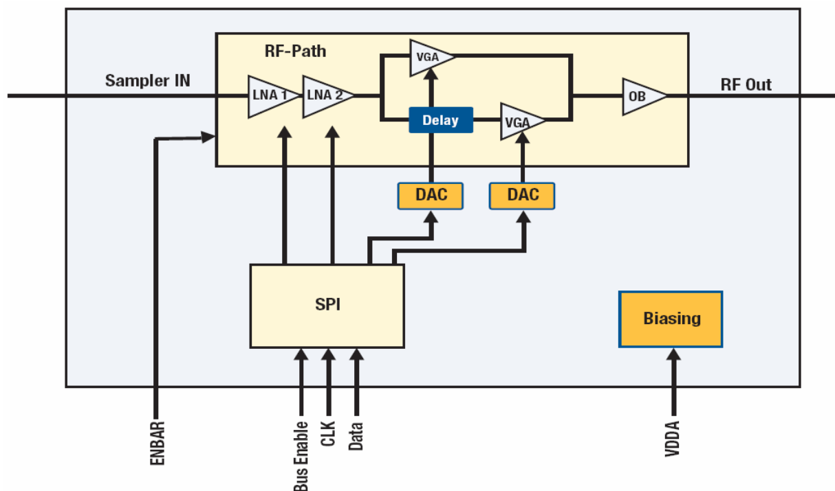
FIGURE 29. BLOCK DIAGRAM
