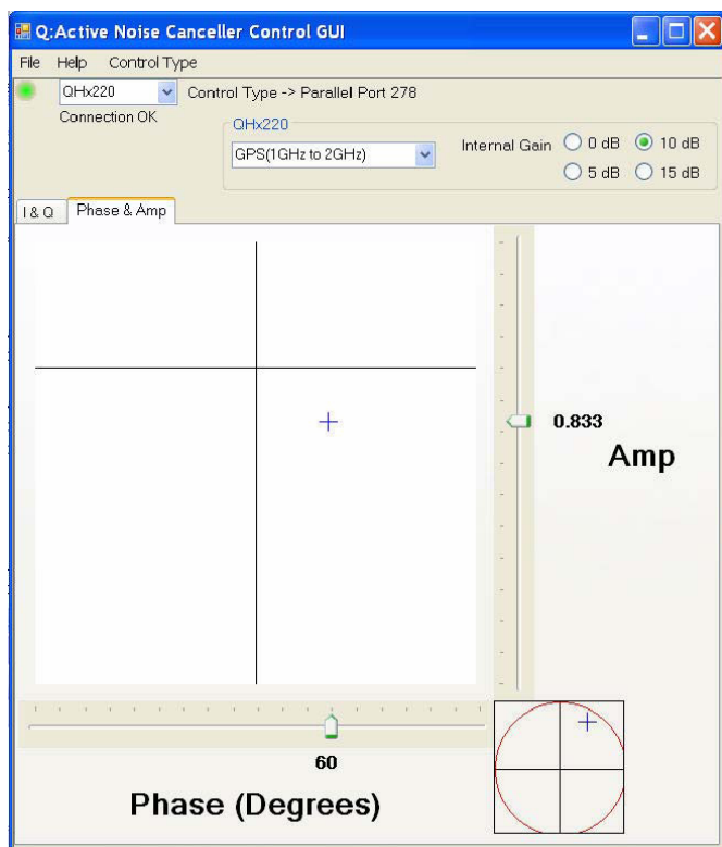
FIGURE 32. SOFTWARE GUI
