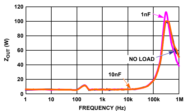
FIGURE 54. Z_{OUT} vs FREQUENCY
