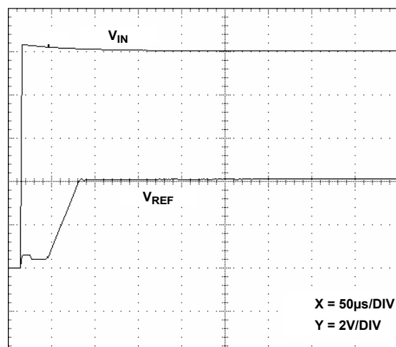
FIGURE 39. TURN-ON TIME
