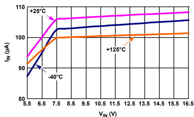
FIGURE 45. I_{IN} vs V_{IN} , 3 TEMPERATURES
