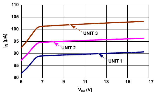
FIGURE 2. I_{IN} vs V_{IN} , 3 UNITS
