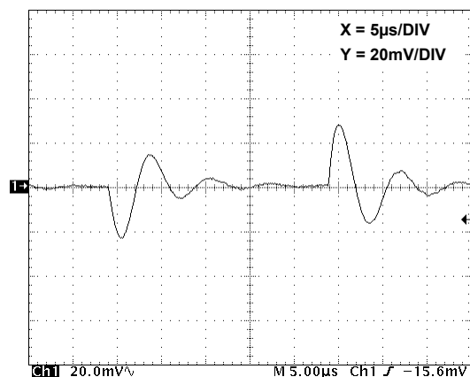
FIGURE 10. LINE TRANSIENT RESPONSE, 0.001µF LOAD CAPACITANCE
