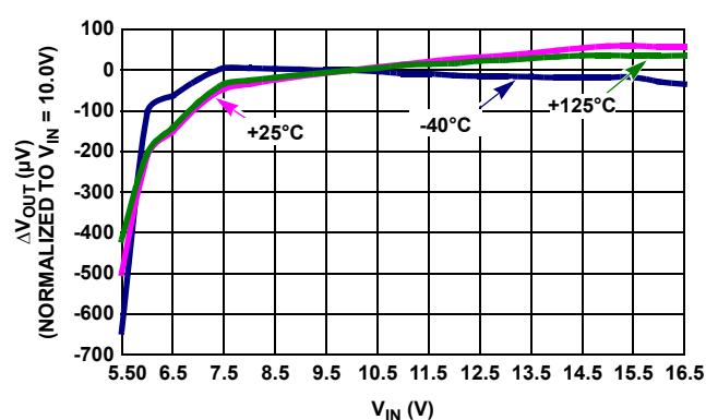
FIGURE 47. LINE REGULATION OVER-TEMPERATURE
