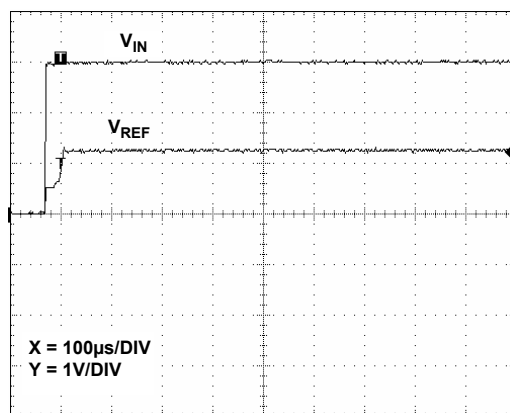
FIGURE 11. TURN-ON TIME
