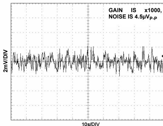
FIGURE 13. V_{OUT} NOISE, 0.1Hz TO 10Hz
