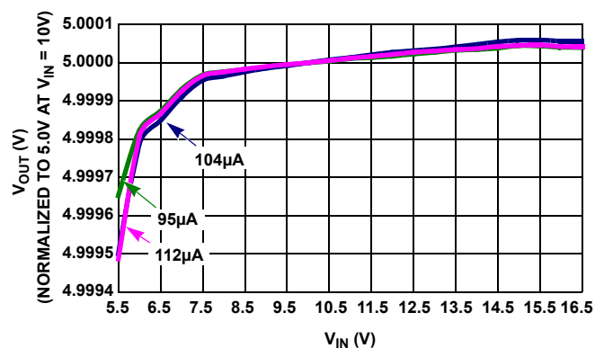
FIGURE 46. LINE REGULATION
