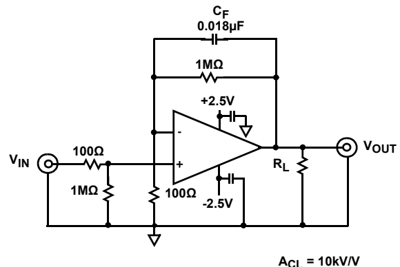
FIGURE 36. HIGH GAIN, PRECISION DC-COUPLED AMPLIFIER
