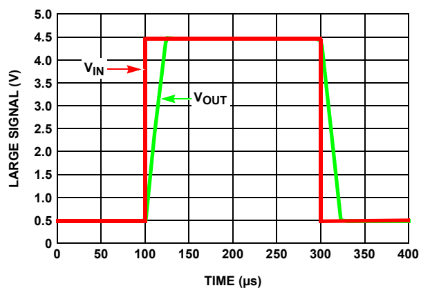
FIGURE 49. SIMULATED LARGE SIGNAL STEP RESPONSE (4V)
