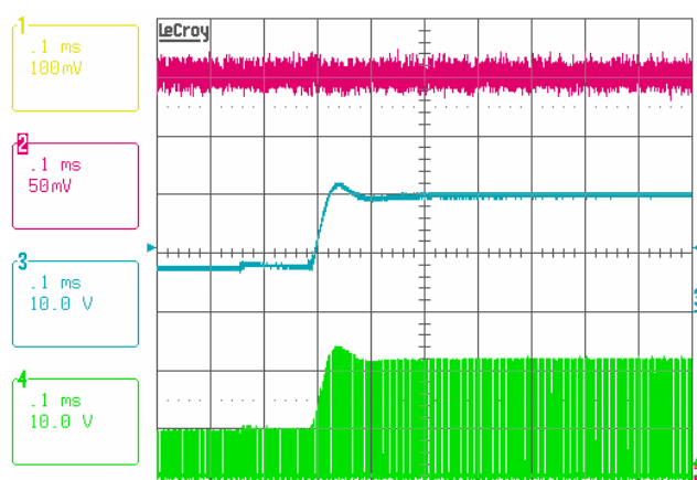
FIGURE 30. V_{IN} TRANSIENT TEST, V_{IN} = 8 \rightarrow 19V , I_O = 2A , V_{ID} = 1.1V , Ch2: V_O , Ch3: V_{IN} , Ch4: PHASE
