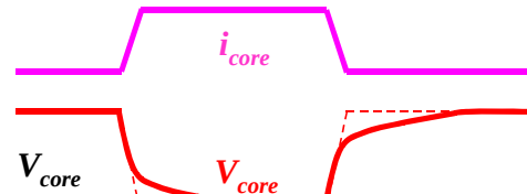
FIGURE 12. LOAD TRANSIENT RESPONSE WHEN C_n IS TOO LARGE
