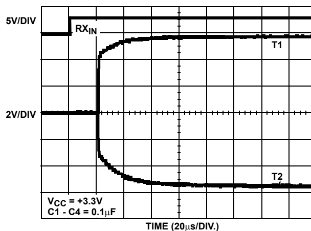
FIGURE 6. TRANSMITTER OUTPUTS WHEN EXITING POWERDOWN (ICL3217 ONLY)
