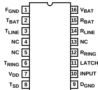
ISL5571A TOP VIEW
