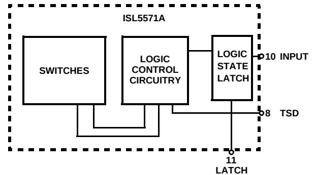
FIGURE 2. BLOCK DIAGRAM OF LOGIC CONTROL
