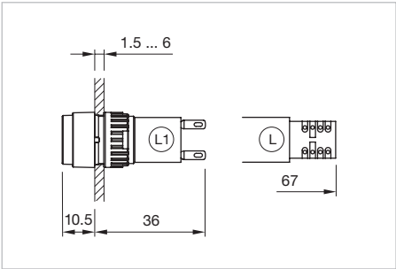
Dimensions [mm] L = Solder terminal, L1 = Solder terminal 2.8 x 0.5 mm
