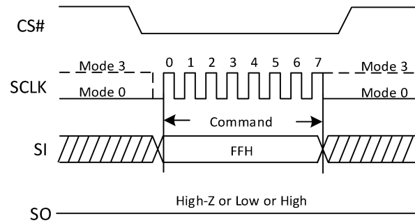
Figure25. RESET (FFh) Diagram
