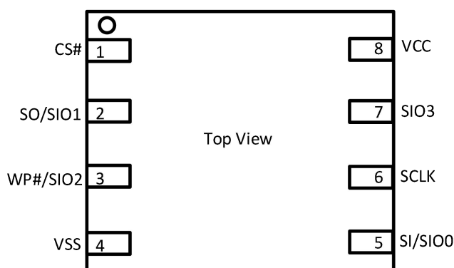
Figure1. Pin Assignment
