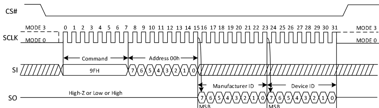
Figure15. Read ID Sequence Diagram
