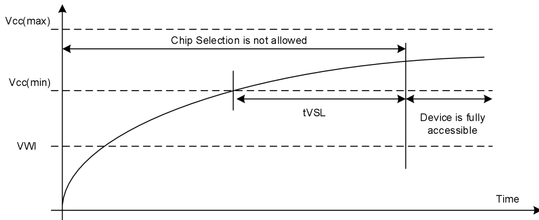
Figure26. Power-On Timing
