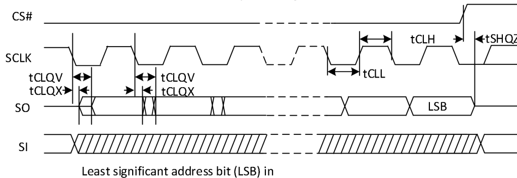
Output Timing
