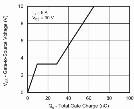
Gate Charge
