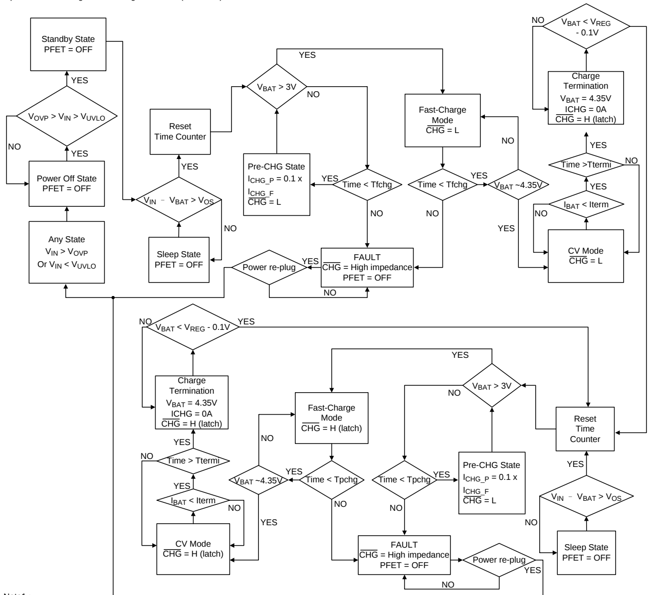
Operation State Diagram for Charger Function (RT9527H)
