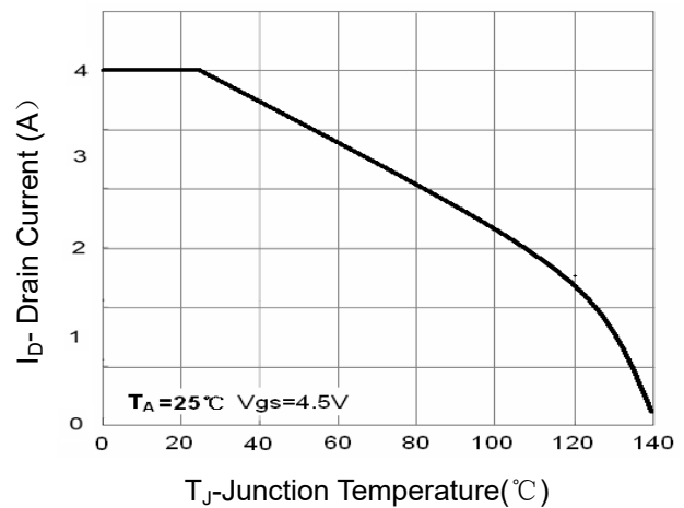
Figure 4 Drain Current
