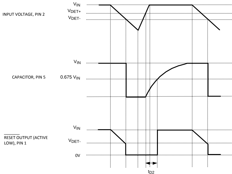
Figure 1. Timing Waveforms
