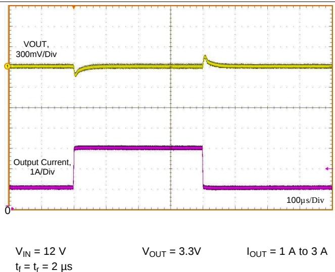
Figure 41. Load Transient
