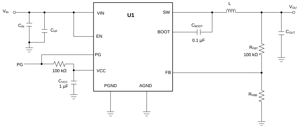
Figure 48. Circuit for Application Curves
