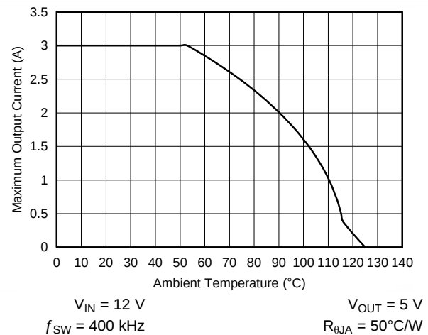
Figure 23. Maximum Output Current vs Ambient Temperature
