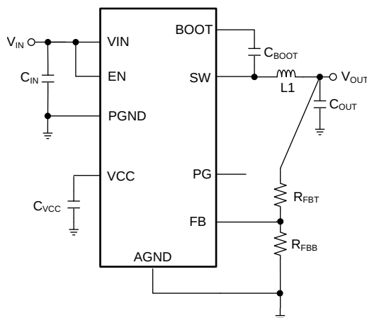
Simplified Schematic
