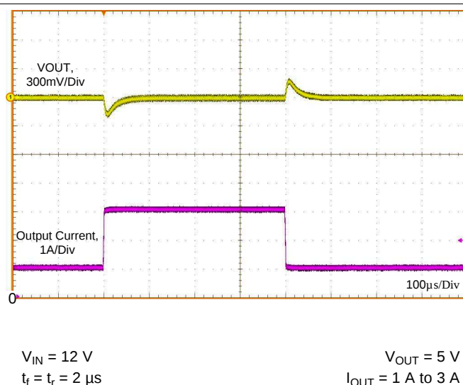
Figure 35. Load Transient
