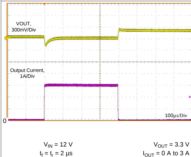
Figure 40. Load Transient
