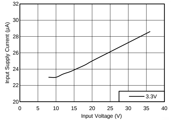
Figure 37. Input Supply Current
