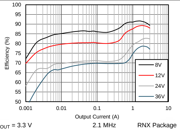
Figure 29. Efficiency
