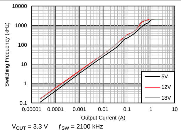
Figure 39. Switching Frequency vs Output Current
