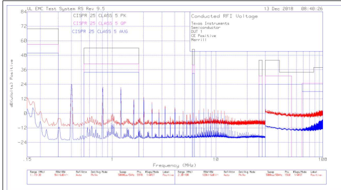
Figure 42. Conducted EMI
