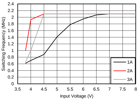
Figure 17. Typical Switching Frequency in Dropout Mode V OUT = 3.3 V, f SW = 2.1 MHz
