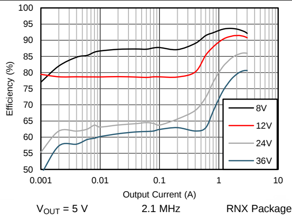
Figure 28. Efficiency
