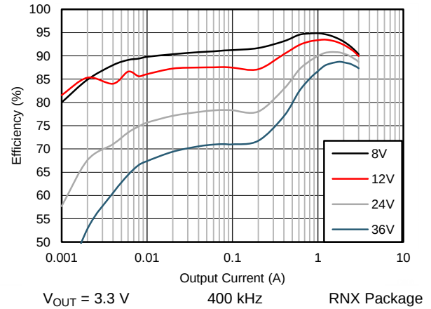
Figure 25. Efficiency
