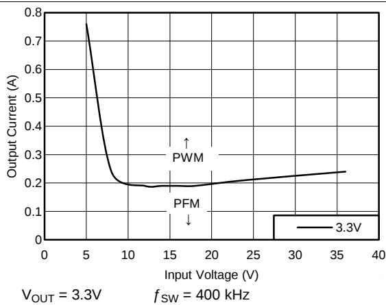
Figure 38. Mode Change Thresholds
