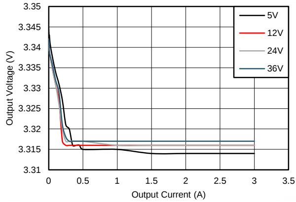
Figure 36. Line and Load Regulation
