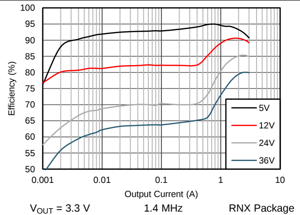
Figure 27. Efficiency
