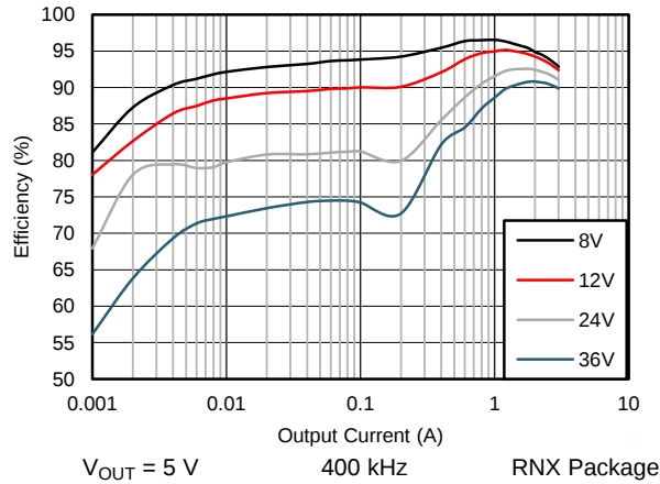
Figure 24. Efficiency
