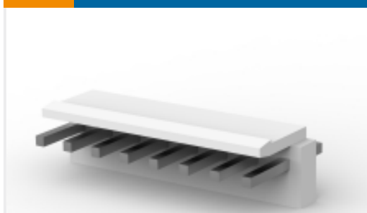
TE Part #2410284-8 3.96 EP HDR ASY 08P NO PEG, GW
