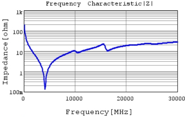
GJM0335C2A8R4DB01 |Z| DCOV, 25degC
