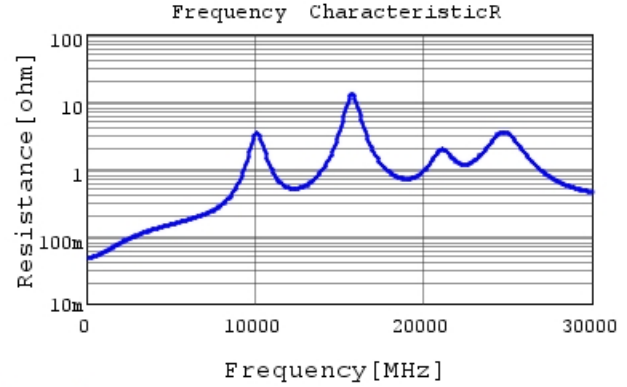
GJM0335C2A8R4DB01 R DCOV, 25degC
