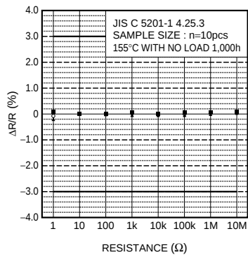
Fig.12 Endurance
