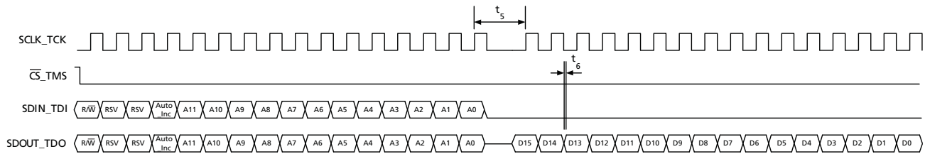
Figure 4-28: Read Mode
