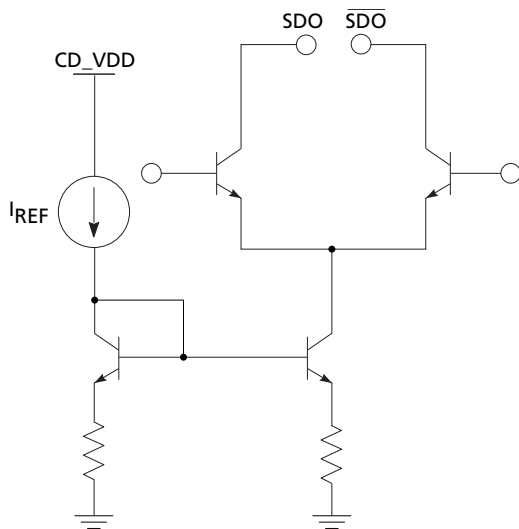
Figure 3-1: Differential Output Stage (SDO/SDO)
