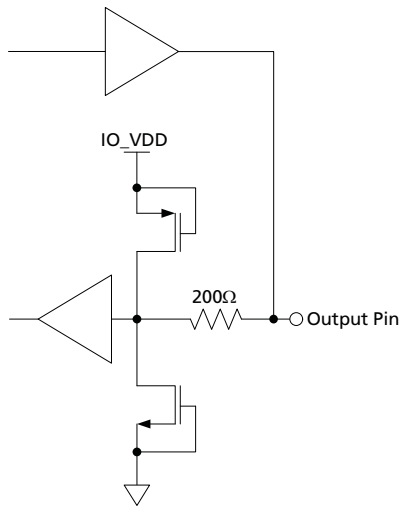
Figure 3-7: Bidirectional Digital Input/Output Pin with programmable drive strength. These pins are configured to output at all times except in reset mode. (LOCKED, AUDIO_INT, SDOU_TDO, TDO)
