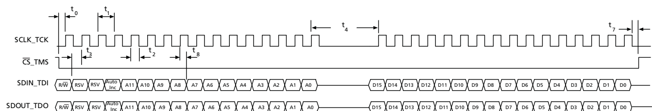
Figure 4-27: Write Mode
