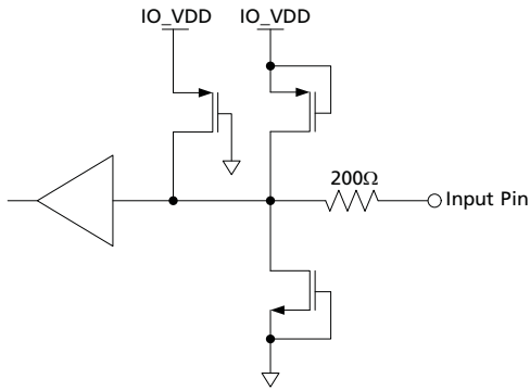
Figure 3-5: Digital Input Pin with weak pull-up - maximum pull-up current <110μA (ACLK1, ACLK2, AIN_7/8, AIN_5/6, AIN_3/4, AIN_1/2, CS_TMS, GRP1_EN/DIS, GRP2_EN/DIS, IOPROC_EN/DIS, SDO_EN/DIS, TMS, WCLK1, WCLK2)
