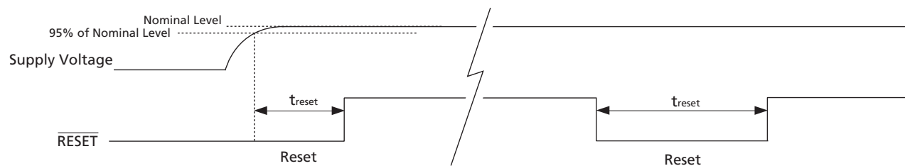
Figure 4-30: Reset Pulse
