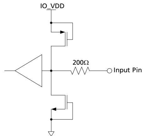
Figure 3-2: Digital Input Pin (20bit/10bit, ANC_BLANK, DETECT_TRS, DVB_ASI, RATE_SEL, SMPTE_BYPASS, TIM_861, F/DE, H/HSYNC, PCLK, V/VSNC)
