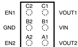
TPS718xx, TPS719xx YZC Package 6-BALL WCSP (TOP VIEW)
