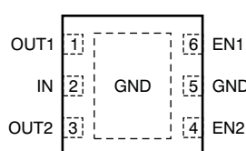
TPS718xx, TPS719xx DRV Package 2mm × 2mm SON (TOP VIEW)
