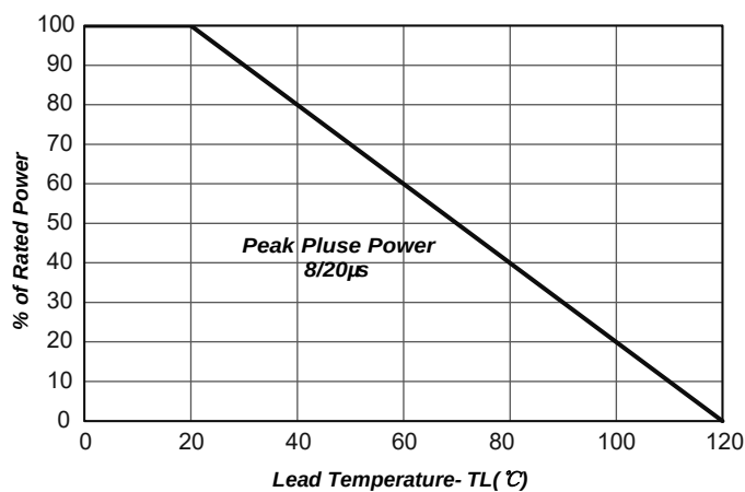
Fig2.Power Derating Curve
