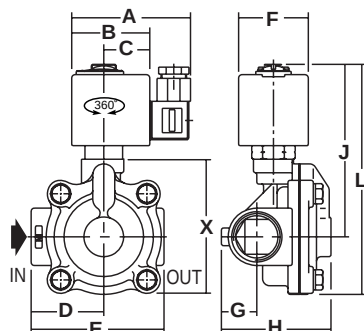
TYPE 03 Prefix "SC" Solenoid Epoxy moulded IEC 335 / ISO 4400 IP65
