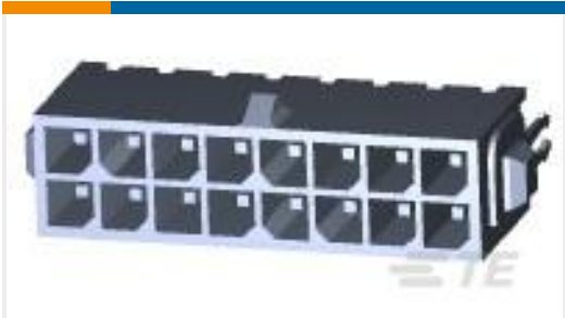
TE Part #4-794680-6 16P MICRO MNL ASSY,VRT,THRU LF
