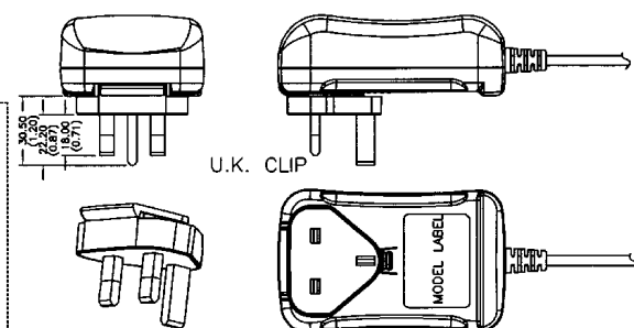
ASSEMBLY FROM HOUSING AND U.K. CLIP
