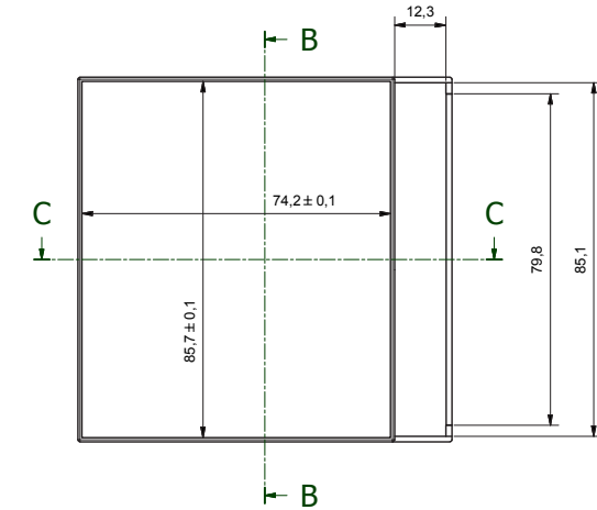
Body enclosure
