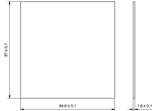
Dimension of PCB
