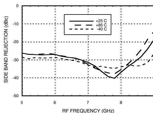
Sideband Rejection vs. Temperature
