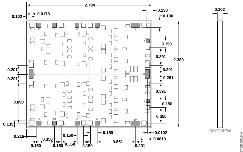
Figure 38. 14-Pad Bare Die [CHIP] (C-14-4)
