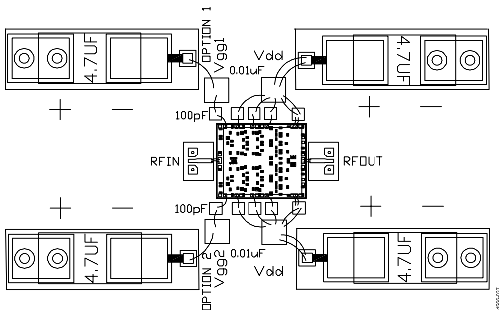
Figure 37. Assembly Diagram
