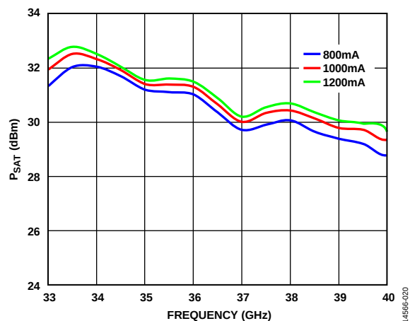
Figure 20. P_{SAT} vs. Frequency at Various Supply Currents
