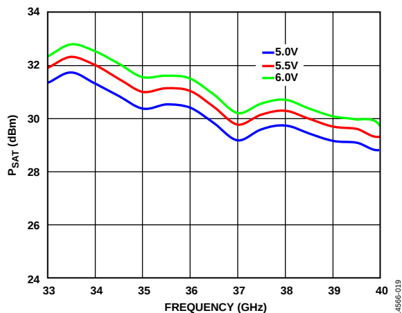
Figure 19. P_{SAT} vs. Frequency at Various Supply Voltages
