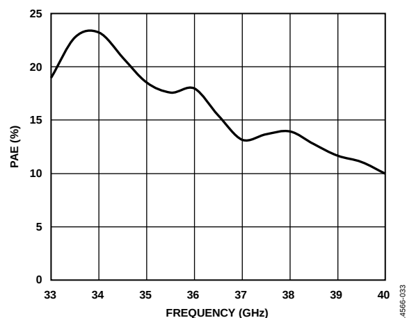
Figure 33. PAE at P_{SAT} vs. Frequency
