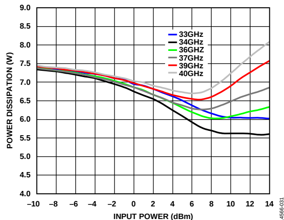
Figure 31. Power Dissipation vs. Input Power for Various Frequencies at T_A = 85^\circ\text{C}
