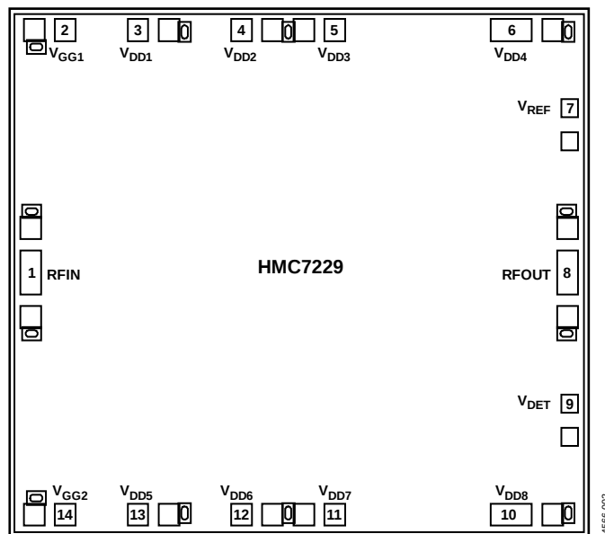
Figure 2. Pad Configuration
