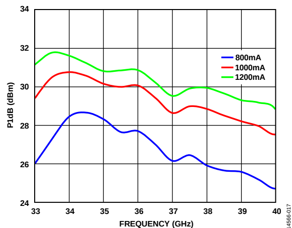
Figure 17. P_{1dB} vs. Frequency at Various Supply Currents
