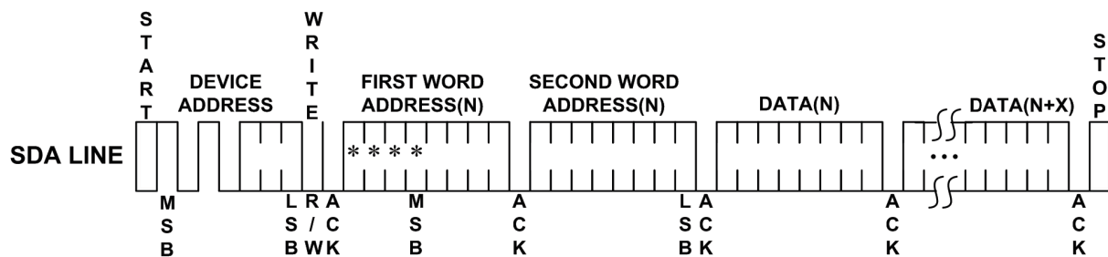
Figure 4: Page Write
