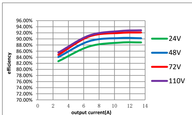
Figure 1: Efficiency vs. load current at 25°C.
