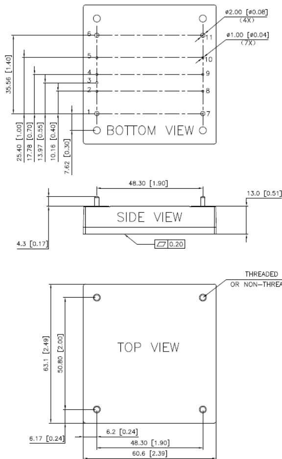
Figure 16: The pin function and mechanical drawing
