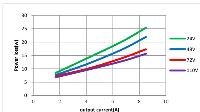
Figure 2: Power loss vs. load current at 25°C.
