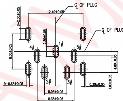
RECOMMENDED PCB LAYOUT TOP VIEW TOLERANCE:±0.05
