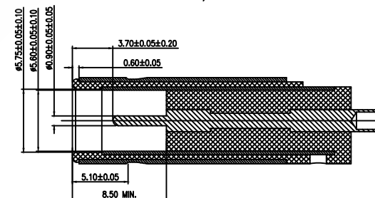
MATING PLUG
