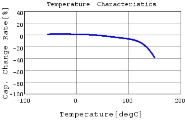
GCJ32DL8EL225KA07 C-Temp. capchange, DC0.0V,
