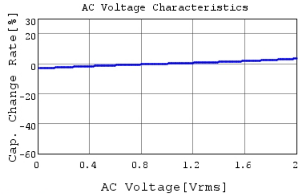
GCJ32DL8EL225KA07 C-AC Voltage capchange, Dc
