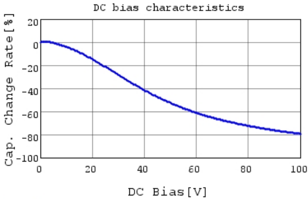
GCJ32DL8EL225KA07 C-DC bias capchange, 25.0c
