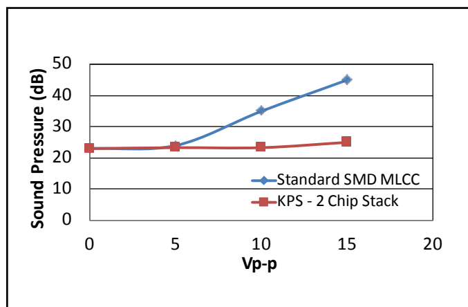
Microphonics – 2220, 47 \mu F, 25 V, X7R
