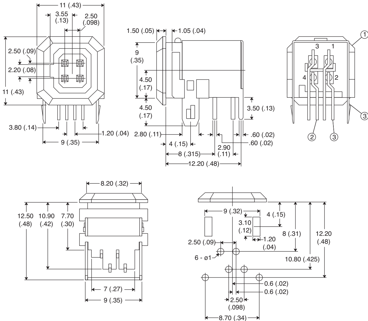
PC Hole Layout (Bottom View)
