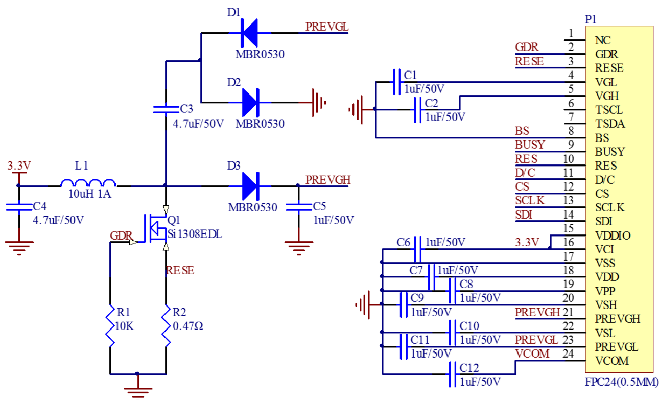
7-5) Reference Circuit
