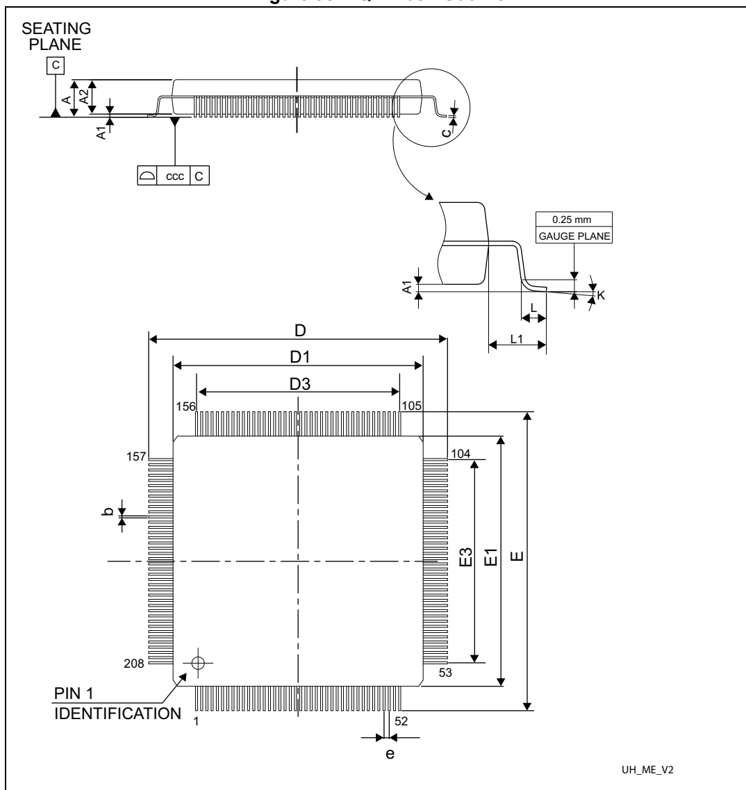
Figure 95. LQFP208 - Outline
