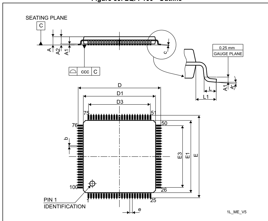
Figure 80. LQFP100 - Outline
