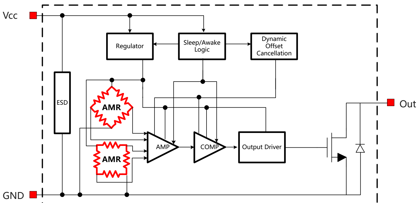
Figure.5 Functional Block Diagram (MR6133 &amp; MR6135)
