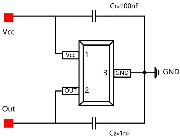
Figure.11 Typical Application Circuit Push Pull Output MR6131 & MR 6132
