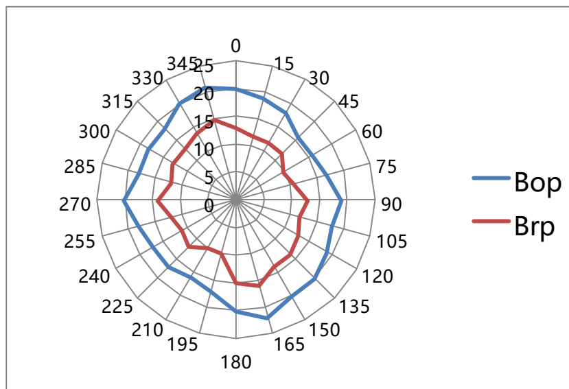
Figure.9 360 Degree Magnetic Characteristics (At V_{CC}=3.6V , T_A=25^\circ C )
