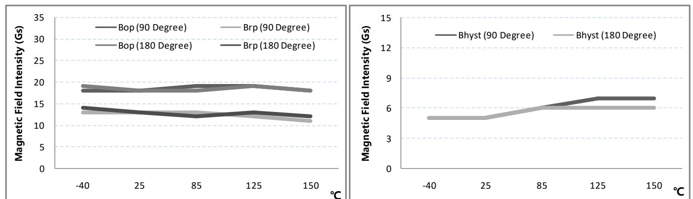
Figure.7 Magnetic Characteristics vs. Temperature (BOP & BRP) (At V_{CC} = 3.6\text{V} ) Magnetic Field @ 90 Degree & 180 Degree
