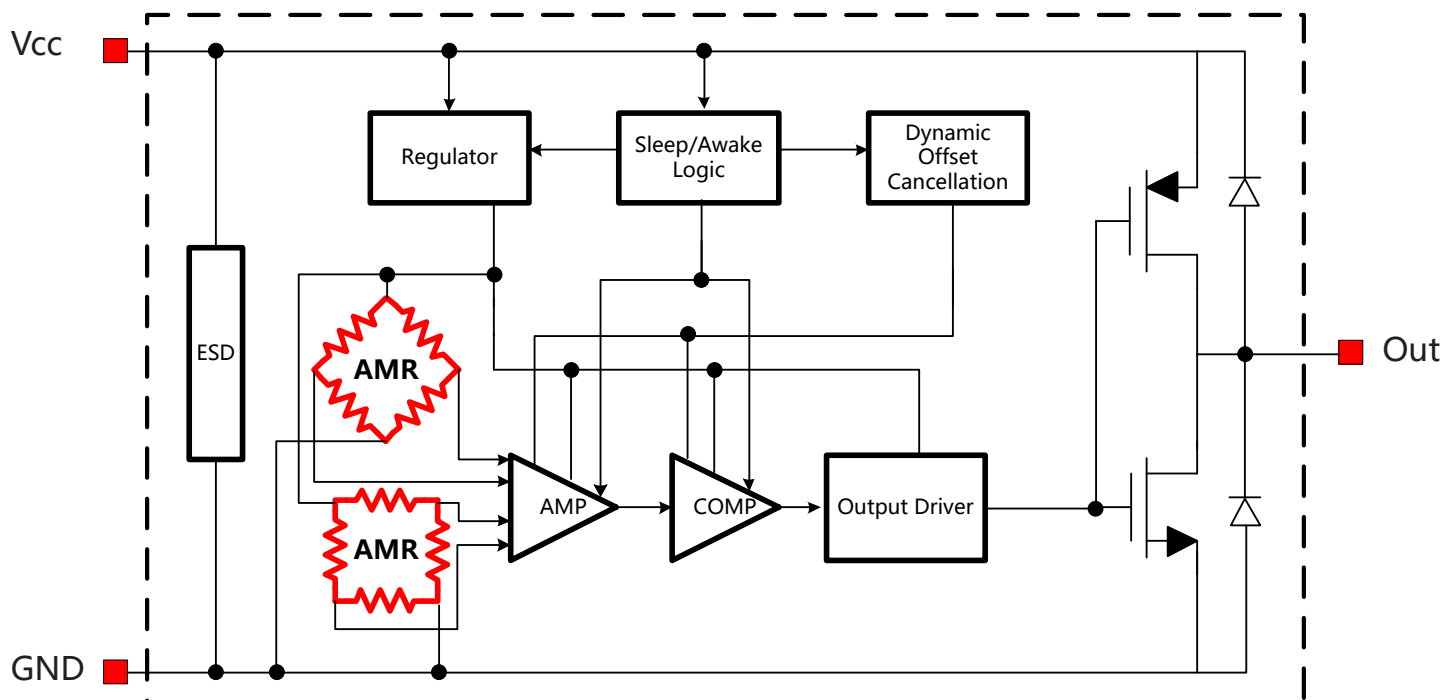
Figure.4 Functional Block Diagram (MR6131 &amp; MR6132)
