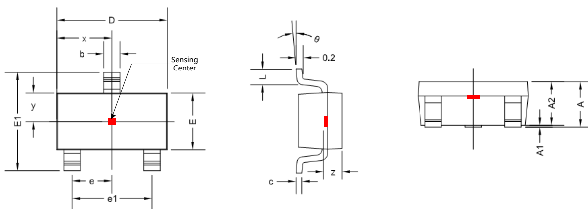
Figure.15 SOT-23 Package Drawing
