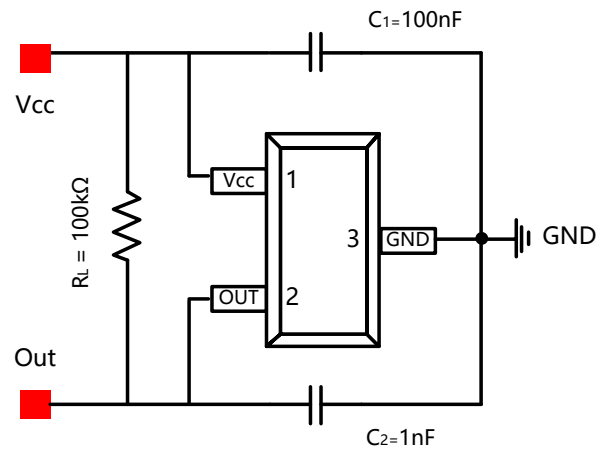
Figure.12 Typical Application Circuit Open Drain Output MR6133 & MR 6135
