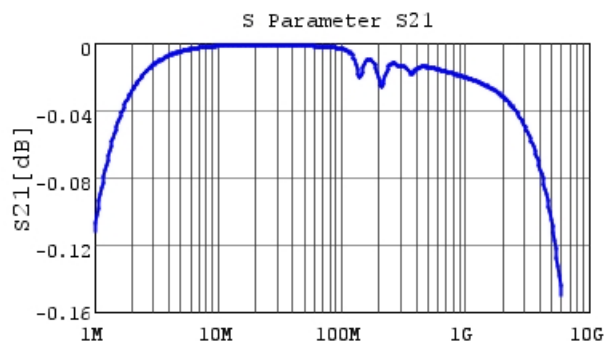
Frequency [Hz] GRT1885C1E103JA02 S21 DCOV, 25degC
