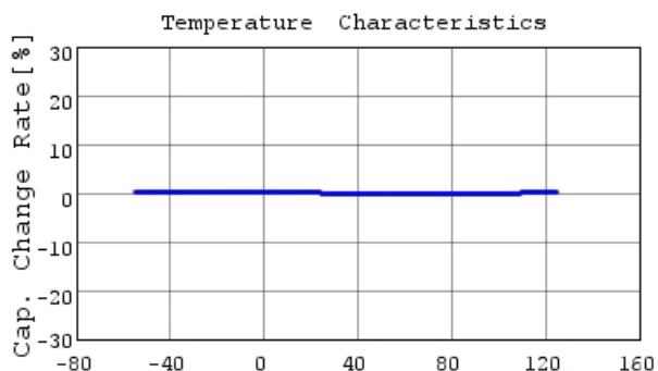
Temperature [degC] GRT1885C1E103JA02 C-Temp. capchange, DCOV, 1
