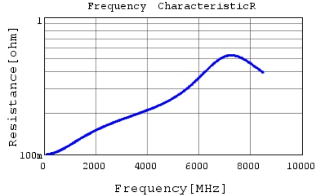
GJM1555C1H5R3BB01 R DCOV, 25degC
