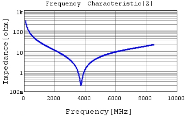
GJM1555C1H5R3BB01 |Z| DCOV, 25degC
