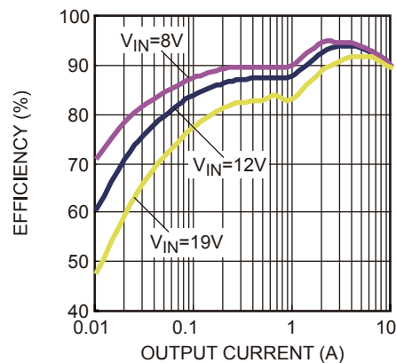
Figure 32 — Efficiency Curve
