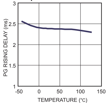
PG Rising Delay vs. Temperature
