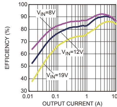
Figure 16 — Efficiency Curve
