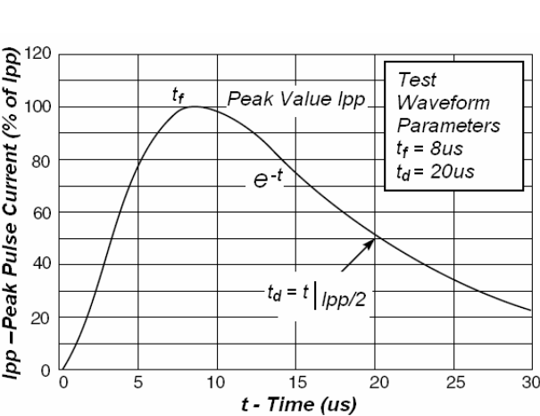
Fig1. Pulse Waveform
