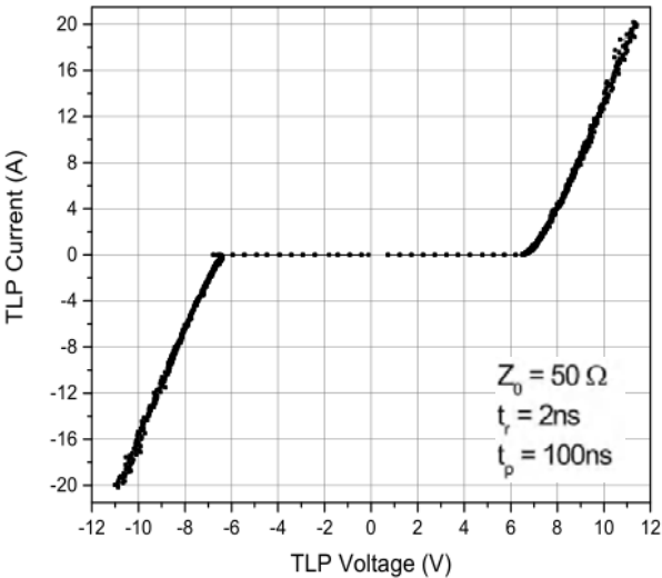
Fig2.TLP Measurement
