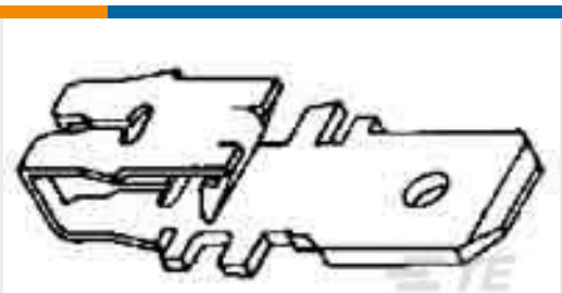
TE Part #2-2293382-5 AMP MONO-SHAPE TAB CONN 5P. GW-V0
