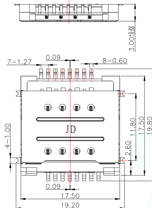
双层 SIM CARD CONNECTOR (短上层)
