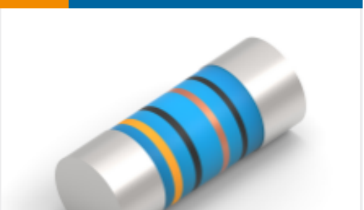
TE Part #4-2176314-7 MELF SMA_A 1K0 1% 50PPM 0102 0.3 W
